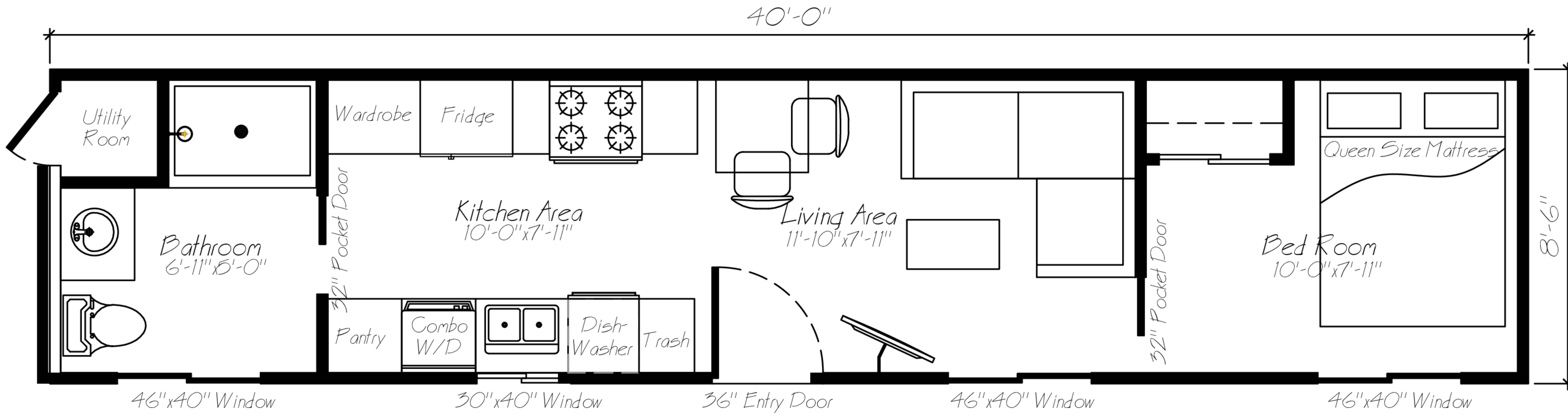
FLOOR PLAN 340 SQFT
